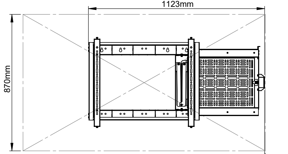
70" SCREEN - CLOSE SCALE 1 : 15
